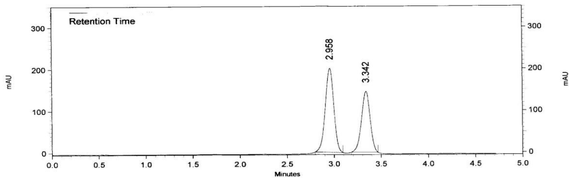
Figure (27): Robustness chromatogram in mobile phase (+5%)
